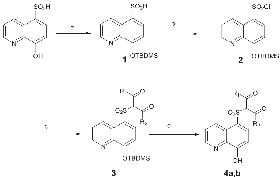
Scheme 1. Reagents and conditions: (a) TBDMS, imidazole, room temp., (b) thionyl chloride, DMF, reflux; (c) NaOMe, \beta -diketones, stirring, 50 °C; and (d) 6N HCl, reflux.
