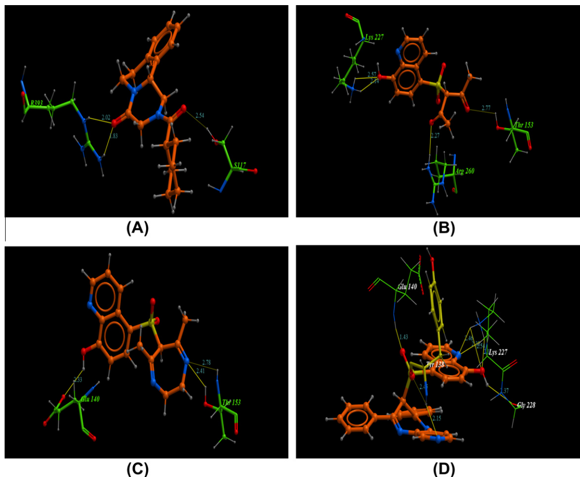
Fig. 2. Molecular docking and binding mode of tested compounds PZQ (reference drug), 4a , 5b , and 7b to the active binding site of TGR receptor.
